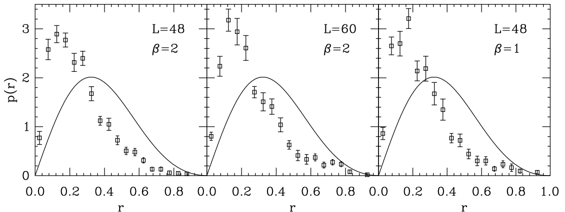
FIG. 4: The distribution of the ratio of the two lowest eigenvalues in the quenched Schwinger model shows that they do not obey the universal distribution given by the chUE.
