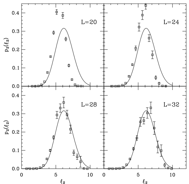
FIG. 7: Rescaled second eigenvalue for N_f = 1 , compared with the prediction of RMT for the N_f = 1 chUE [see Eq. (15) in Ref. 36].
