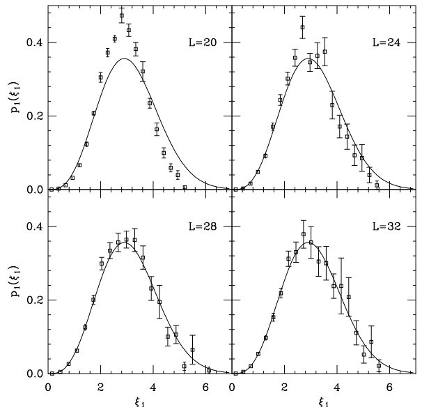
FIG. 6: Comparison of the distribution of the rescaled lowest eigenvalue for N_f = 1 with the prediction of RMT for the N_f = 1 chUE.
