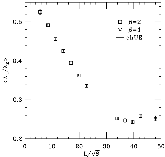
FIG. 5: Expectation value of r = \lambda_1(L, \beta) / \lambda_2(L, \beta) in the quenched Schwinger model as a function of the physical size. The data are not consistent with chUE but do seem to approach a finite limit as L \rightarrow \infty .
