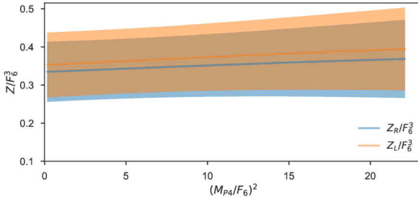
Figure 1: Chimera baryon matrix elements
