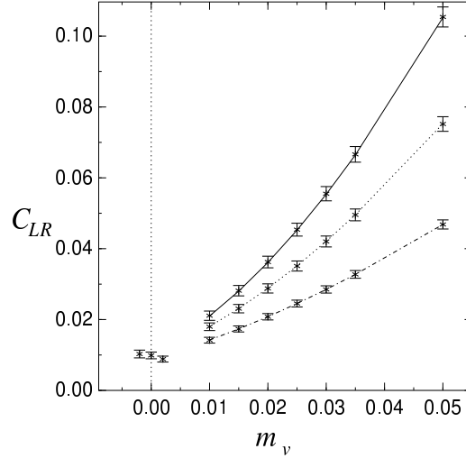
Figure 2: Gauge term in the Higgs effective potential, as a function of valence mass m_v , in a single ensemble. The extrapolations to m_v = 0 are displaced horizontally for clarity.
