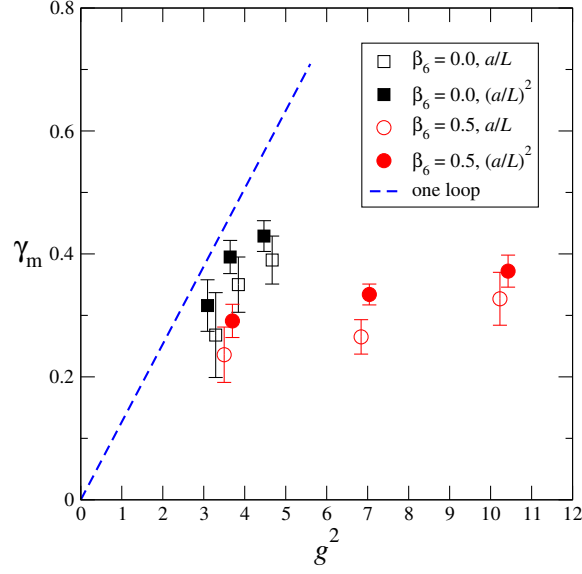
Figure 5: SU(3)/sextet theory [5]: Continuum extrapolations of \gamma_m(g^2) . the black squares and red circles originate from two different lattice actions, while empty (filled) symbols represent linear (quadratic) extrapolations.
