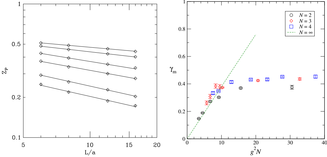
Figure 4: Left: SU(2)/triplet theory [4]. Pseudoscalar renormalization constant Z_P plotted against the size L of the lattice, for bare couplings g_0 ranging from weak (top) to strong (bottom). The fitted log–log slopes give -\gamma_m . Right: \gamma_m(g^2) for the SU(2,3,4) theories, plotted together [6].
