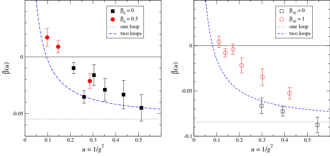
Figure 3: \tilde{\beta} functions for the SU(3)/sextet (left) and SU(4)/decuplet (right) theories [5, 6]. Black squares vs. red circles denote the two different actions used for each theory.
