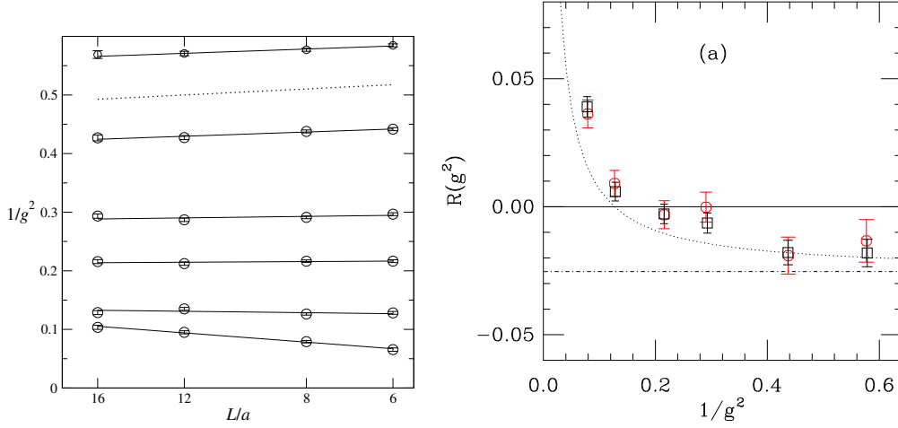
Figure 1: SU(2)/triplet theory [4]. Left: SF coupling vs. size L of the lattice, for bare couplings g_0 ranging from weak (top) to strong (bottom). The fitted slopes give the \tilde{\beta} function. The dotted line has the slope of \tilde{\beta} calculated in the weak coupling limit (one loop). Right: The \tilde{\beta} function extracted from these slopes. The dash-dotted line is the one-loop value and the dotted curve is the two-loop result.
