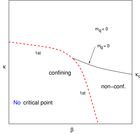
Figure 2: Sketched phase diagram for the SU(3)/sextet theory.
